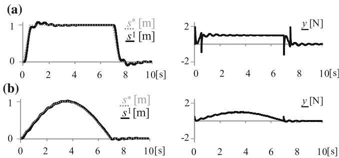
Fig. 5 Controller performance using: a trapezoid signal and b sinuous signal
