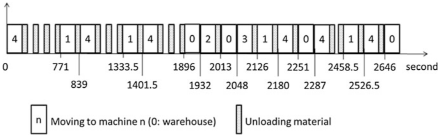
Fig. 3 Robot moving and material unloading
