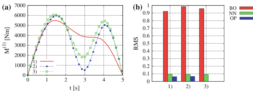
Fig. 6 A comparison of a braking torque courses of the 1st wheel and b RMS values of the tractor roll angle, (1) \delta_{max} = 7^\circ, v_0 = 60 km/h, (2) \delta_{max} = 8.5^\circ, v_0 = 55 km/h, (3) \delta_{max} = 7.8^\circ, v_0 = 57.5 km/h
